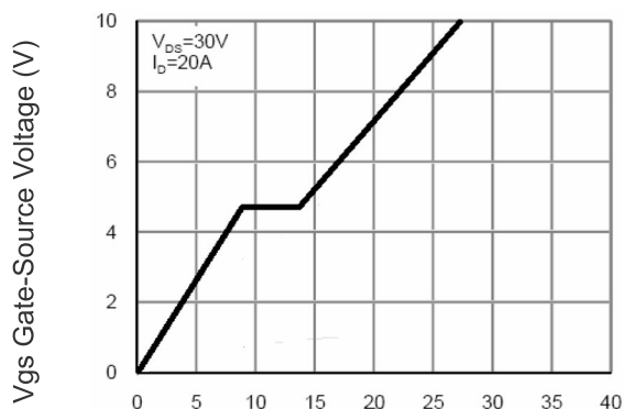
Figure 5 Gate Charge
