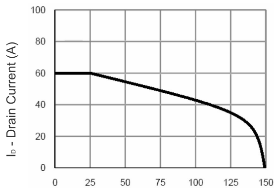
Figure 10 Current De-rating
