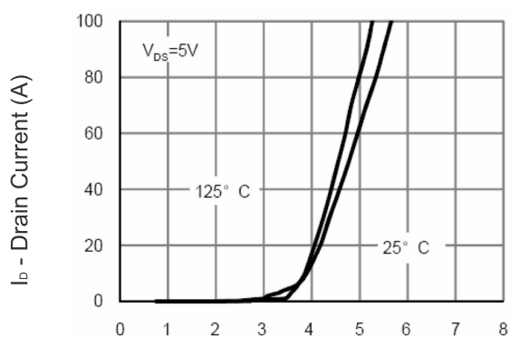
Figure 2 Transfer Characteristics
