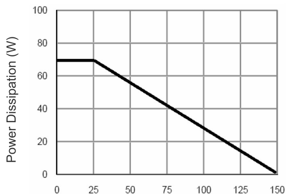
Figure 9 Power De-rating
