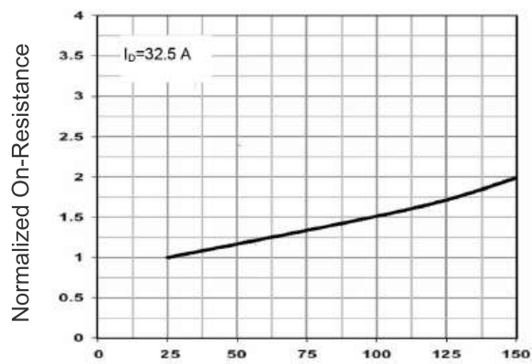
Figure 10 Rdson-Junction Temperature
