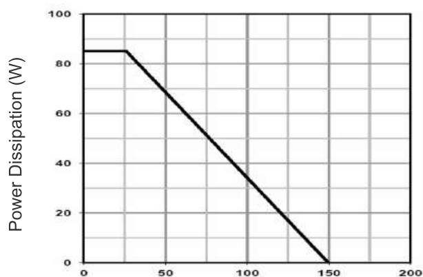
Figure 7 Power De-rating
