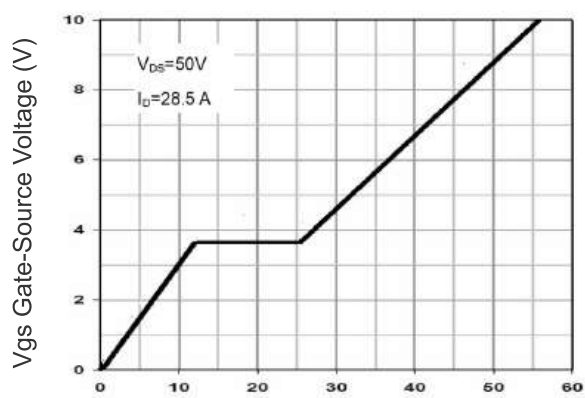
Figure 4 Gate Charge
