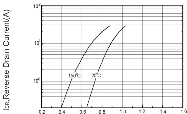
Figure 2 Source-Drain Diode Forward Voltage
