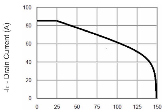
Figure 10 -Current De-rating
