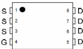
Pin Assignment
