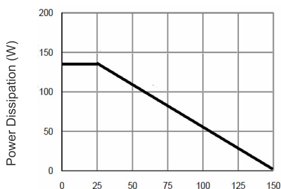
Figure 9 Power De-rating
