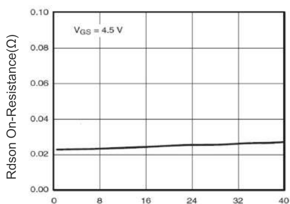
Figure 6 Drain-Source On-Resistance
