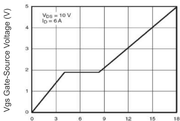
Figure 11 Gate Charge
