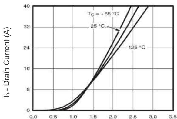
Figure 7 Transfer Characteristics
